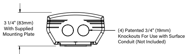
END VIEW
