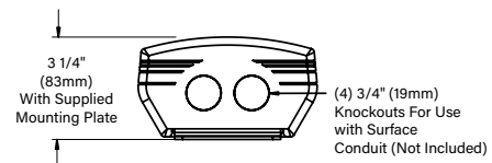
END VIEW
