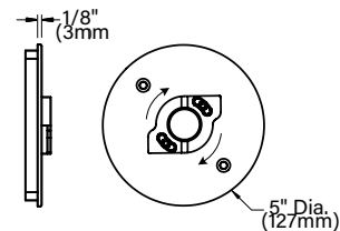
ROUND CAMLOCK™ CANOPY
