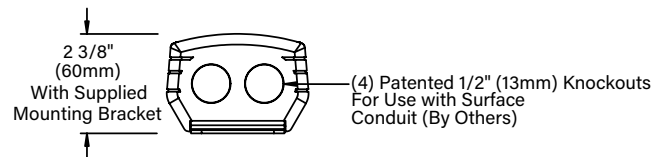
END VIEW
