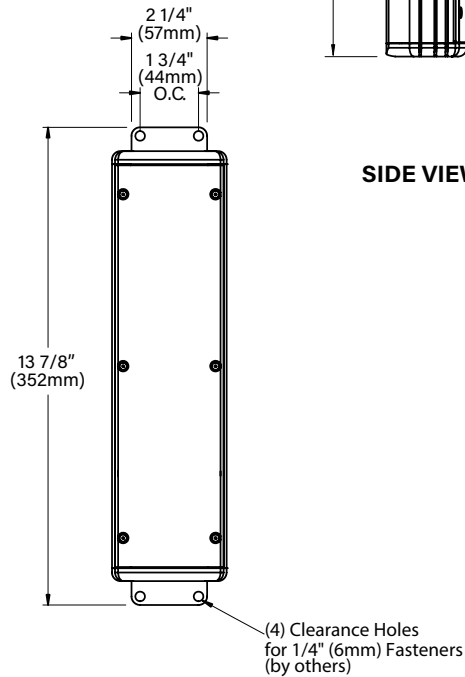
OPTIONAL MOUNTING BRACKET
