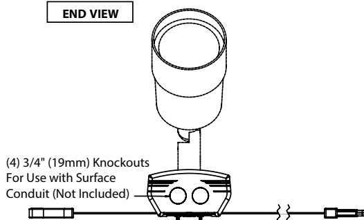
END VIEW
