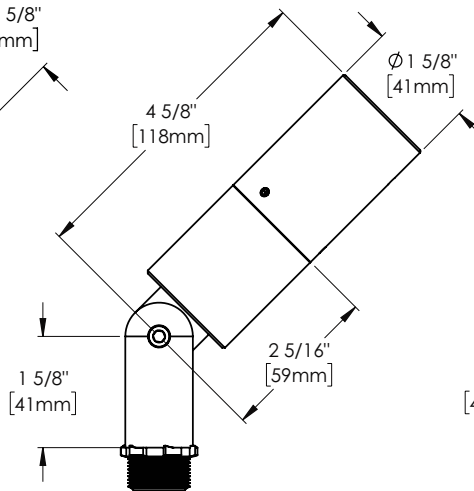
"B/E" CAP
