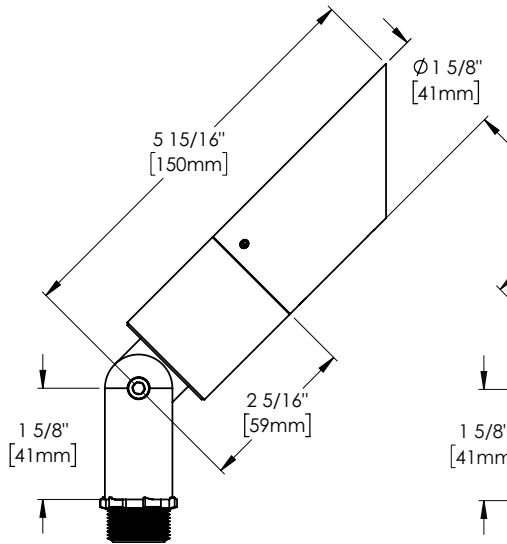
"A/D" CAP
