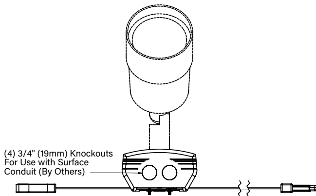
END VIEW
