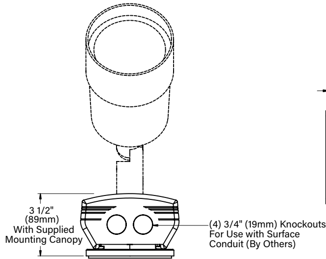
END VIEW
