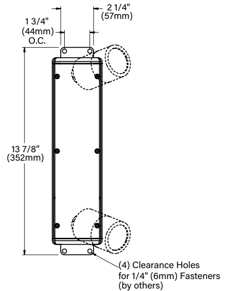
OPTIONAL MOUNTING BRACKET
