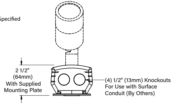
END VIEW
