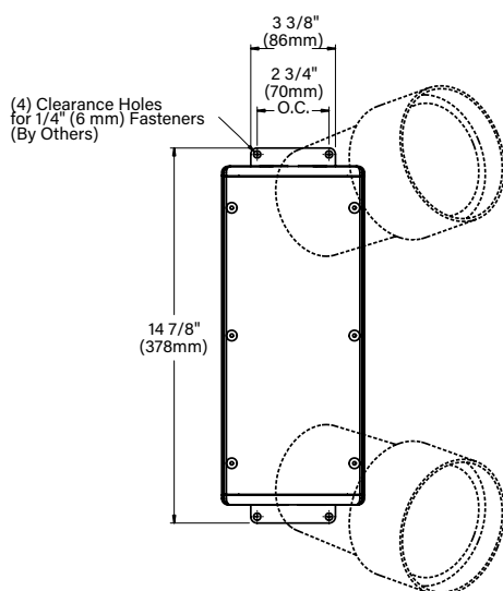
OPTIONAL MOUNTING BRACKET
